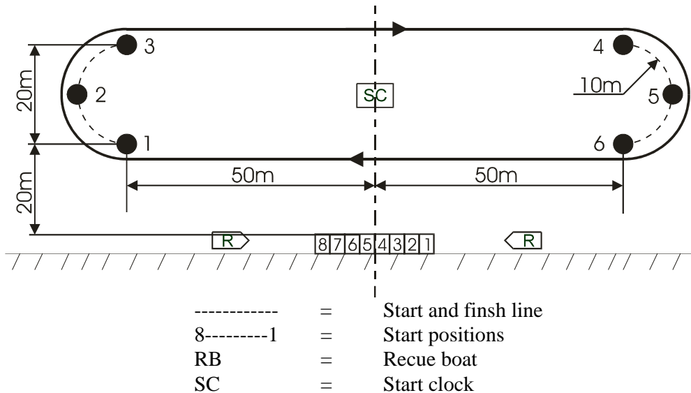
Drawing: 4 FSR-O competition course
